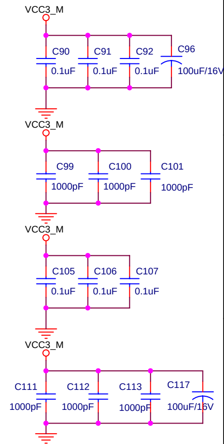
SDRAM DECOUPLING CAPACITORS
