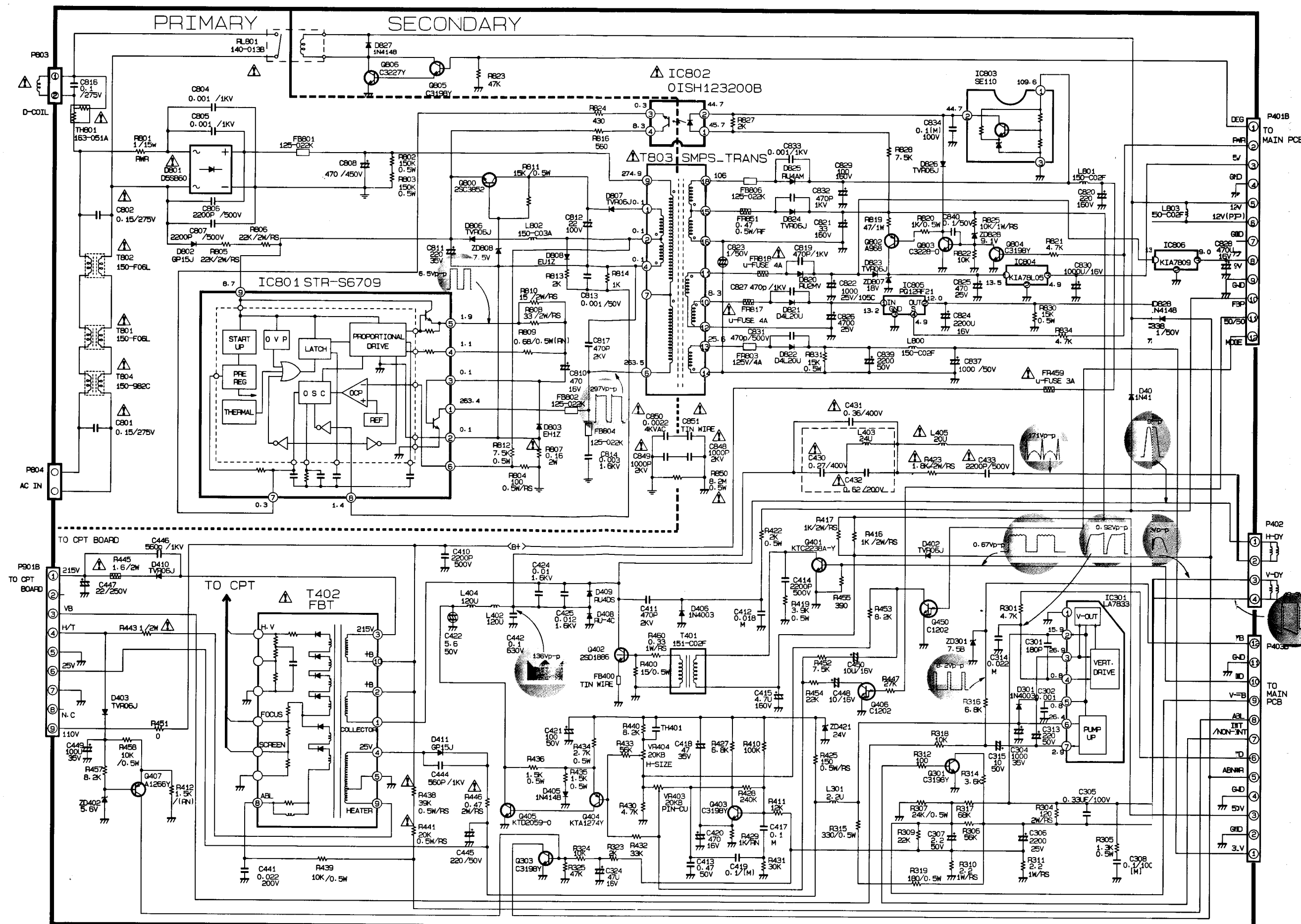
<POWER PCB ASSY>
