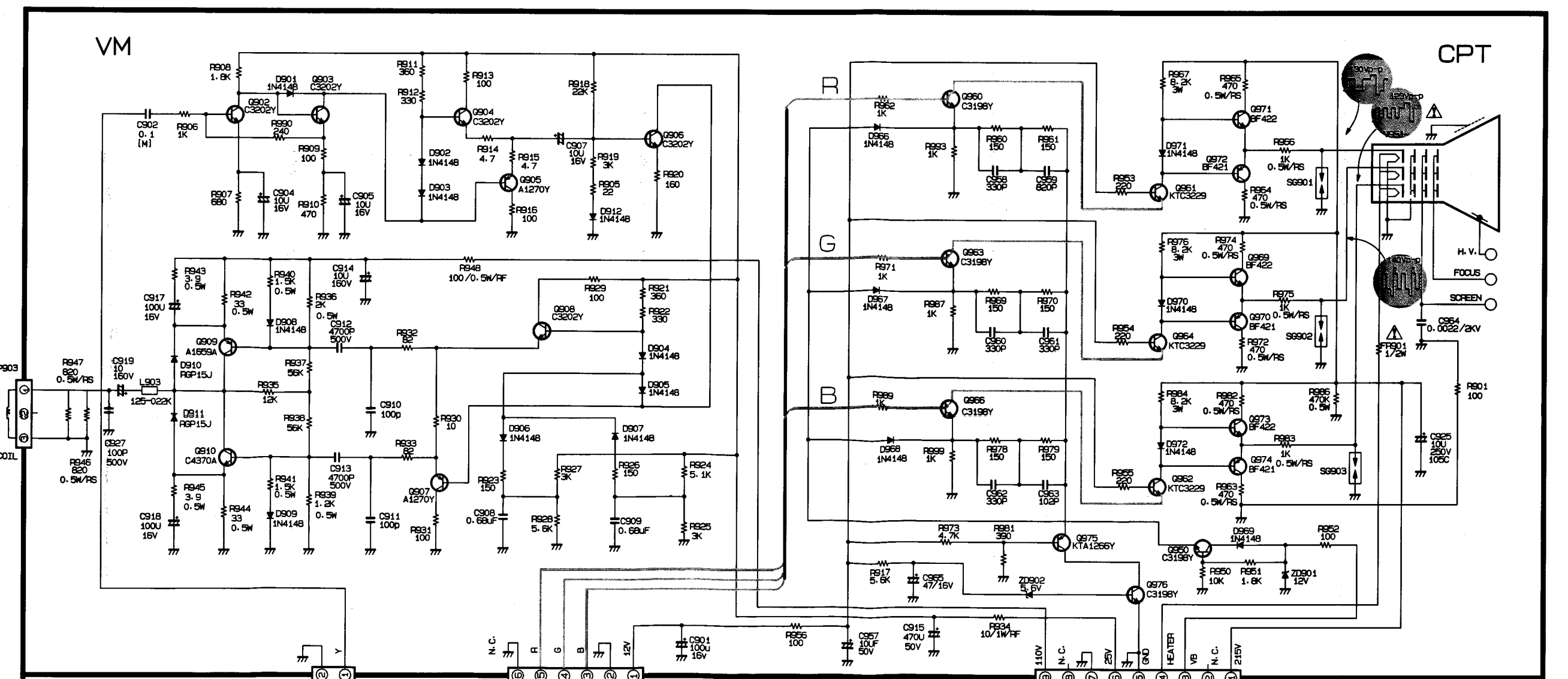
< 29 INCH CPT PCB ASSY >
