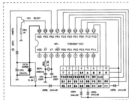
Remote Board JU7.820.1529
