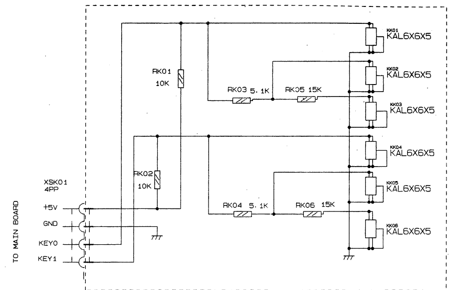
K Board JUC7.820.012
