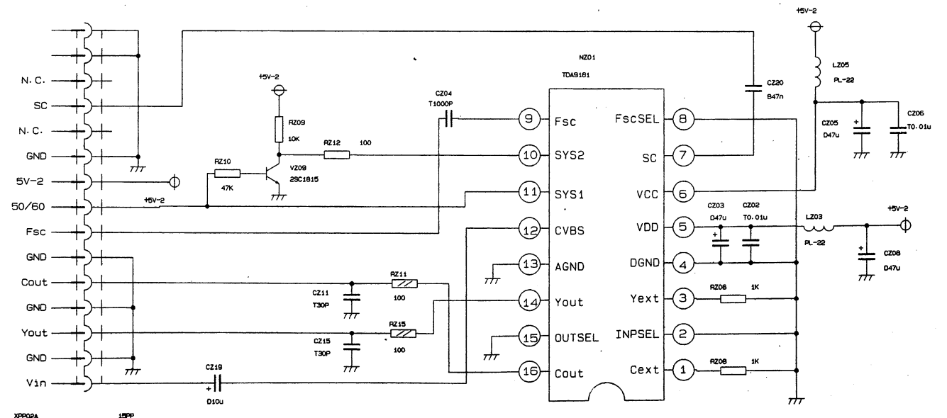
Comb-filter JU7.820.1589-1
