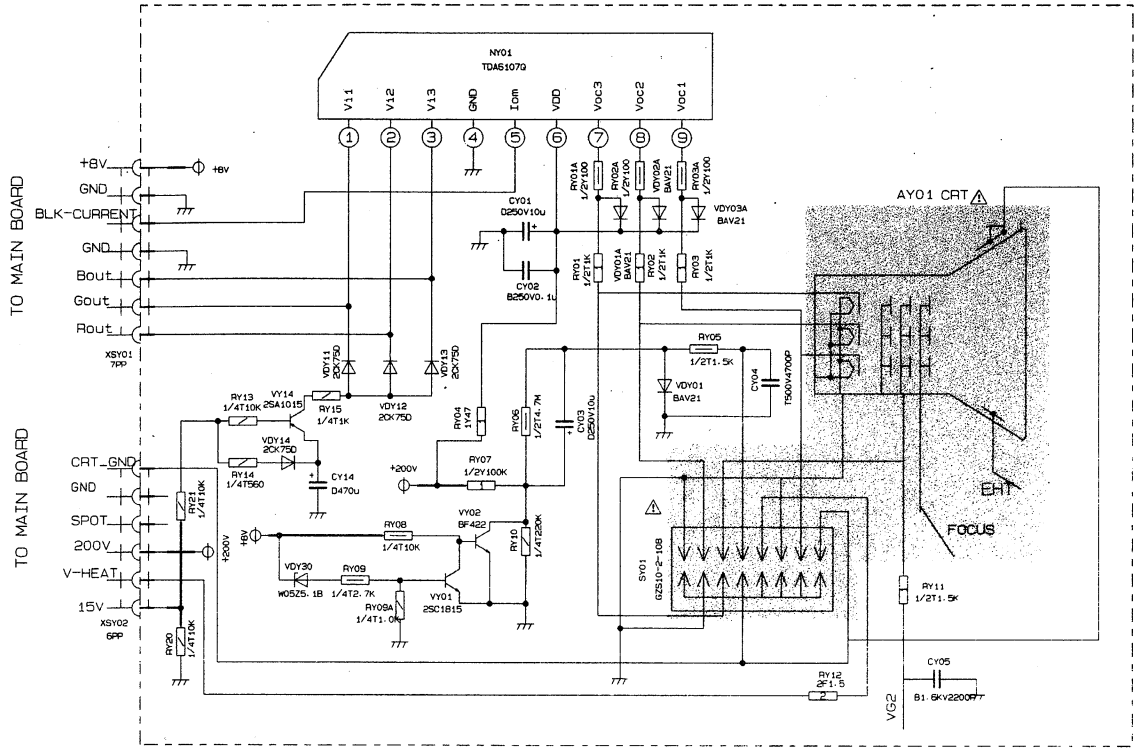
Y BOARD JUC7.820.029
