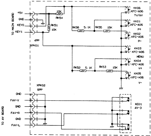
K BOARD JUC7.820.072
