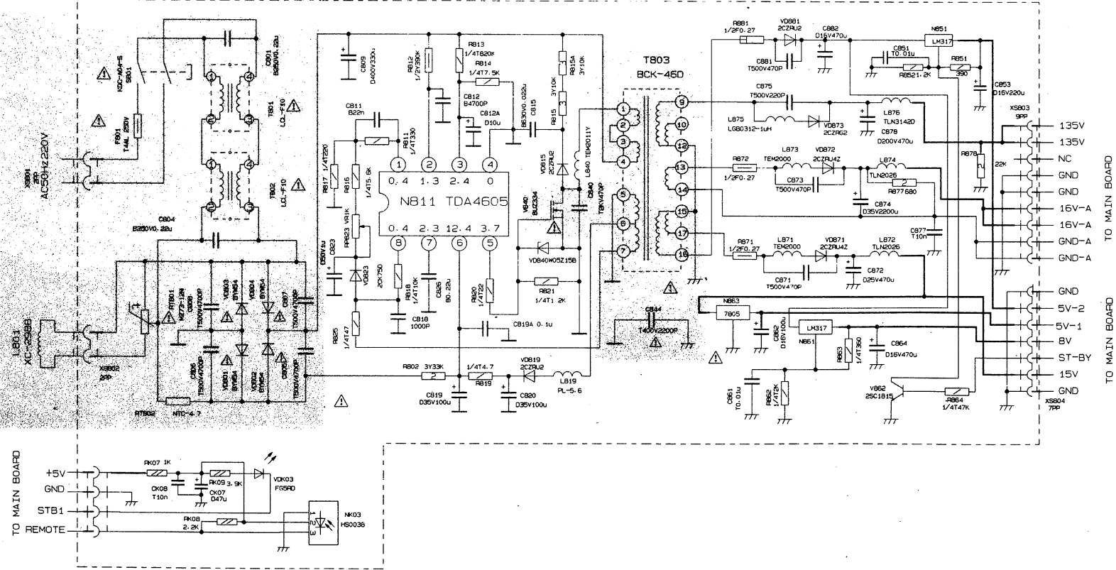
POWER BOARD JUC7.820.028
