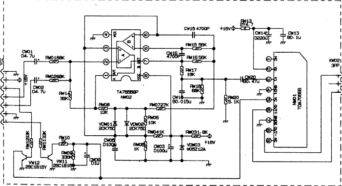
Woofer Board
