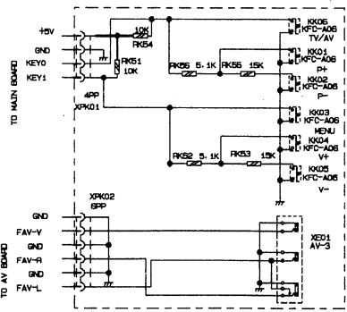
K BOARD JUC7. 820. 027
