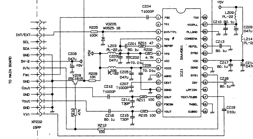
Comb-filter JU7.820.1589
