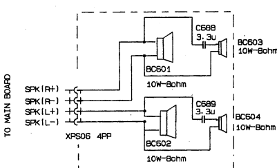
Speaker
