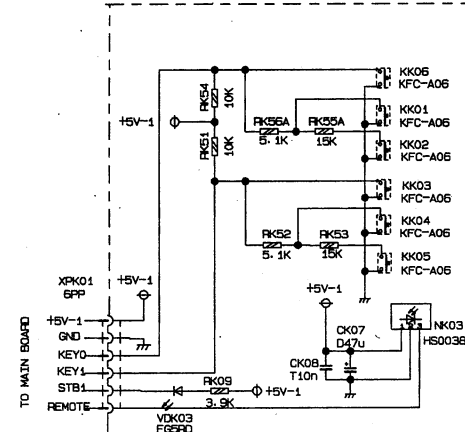
K BOARD JU7.820.1588
