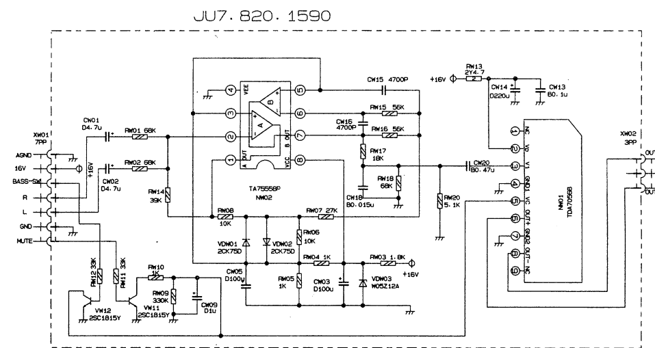
WOOFER BOARD JU7.820.1590
