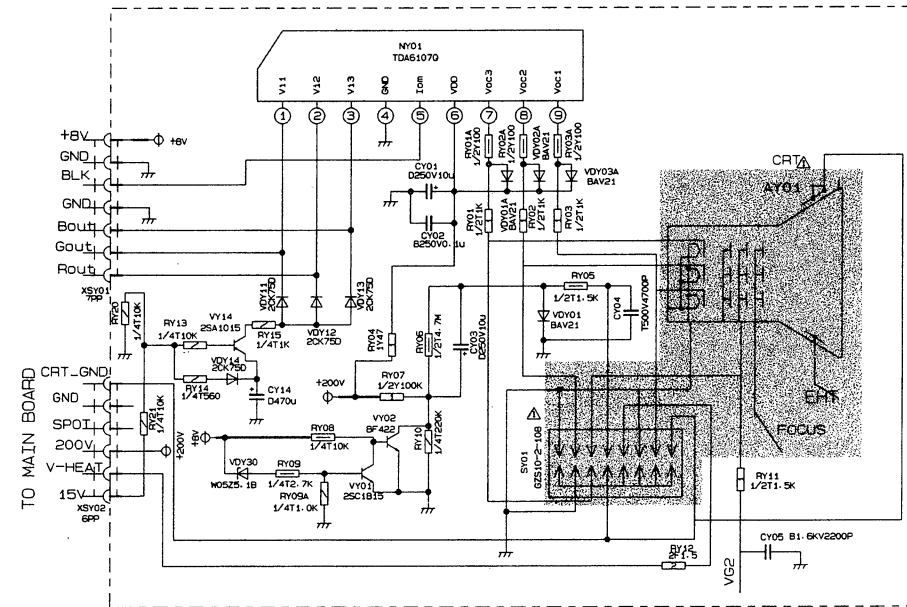
Y BOARD JUC7.820.029
