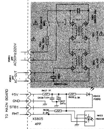
KG BOARD JUC7.820.094
