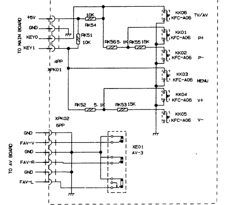
K BOARD JUC7.820.120
