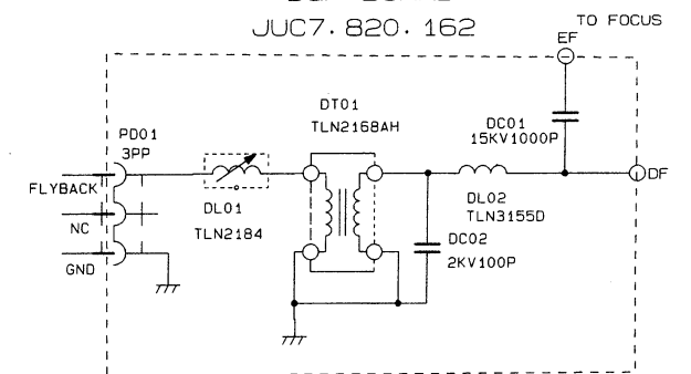
DQF BOARD JUC7.820.162
