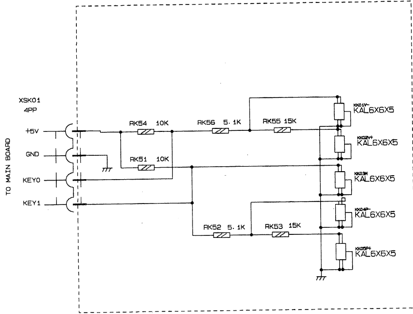
K Board JU7.820.1655
