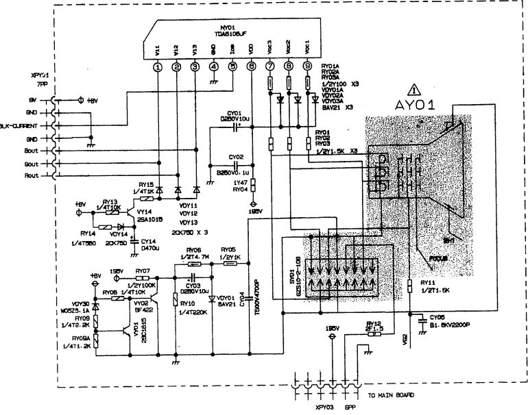
Y Board JU7.820.1586-1
