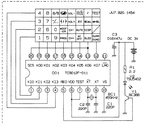
IR REMOTE BOARD
