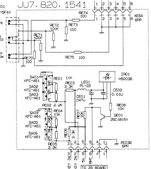
R2516N KZ BOARD
