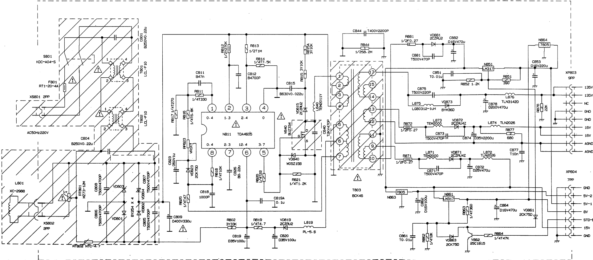
Power Board JU7.820.1587
