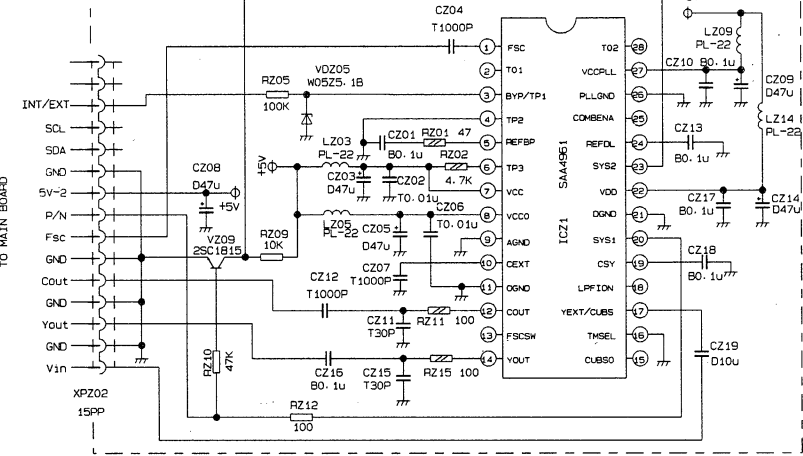
Comb-filter JU7.820.1589
