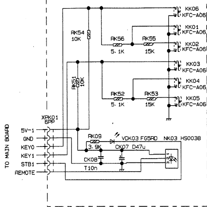
K Board JU7.820.1588
