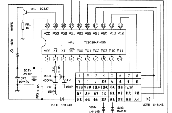
Remote Board JU7.820.1529
