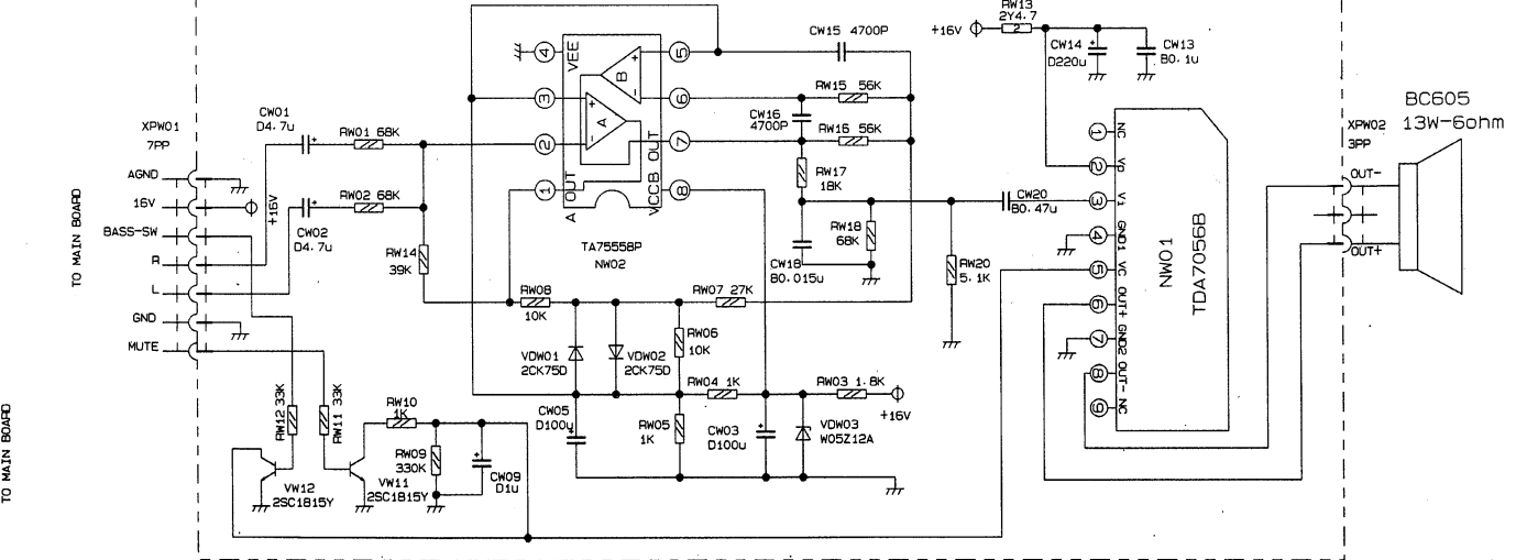
Woofer Board JU7.820.1590
