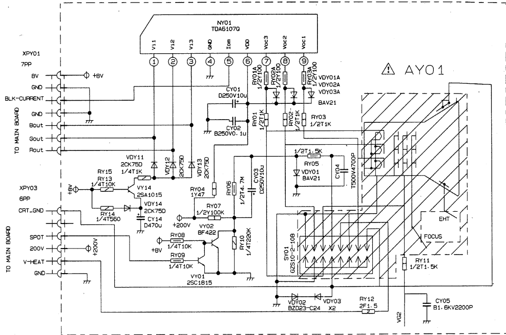
Y Board JU7.820.1586
