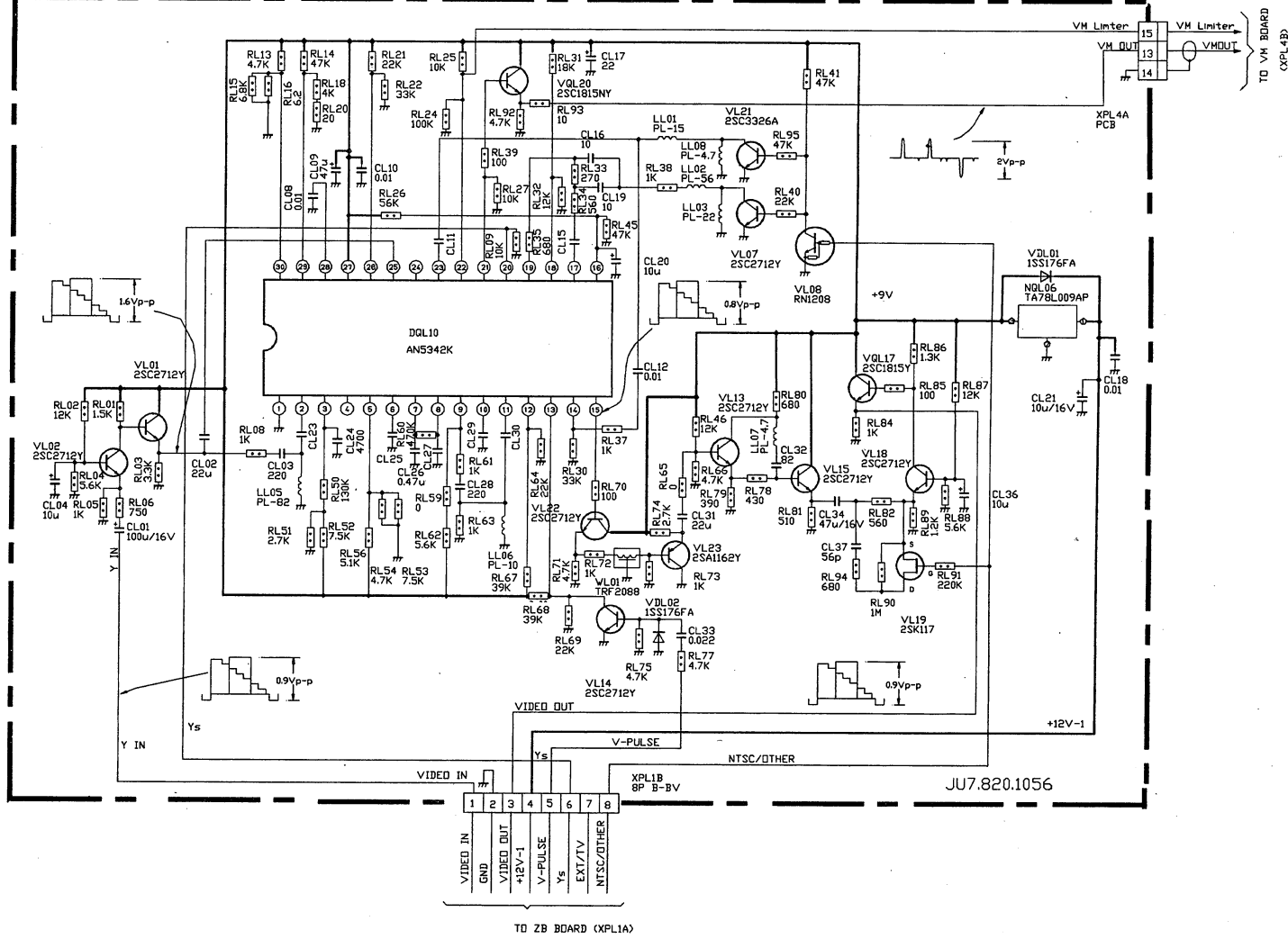
U303 LT BOARD PB3116
