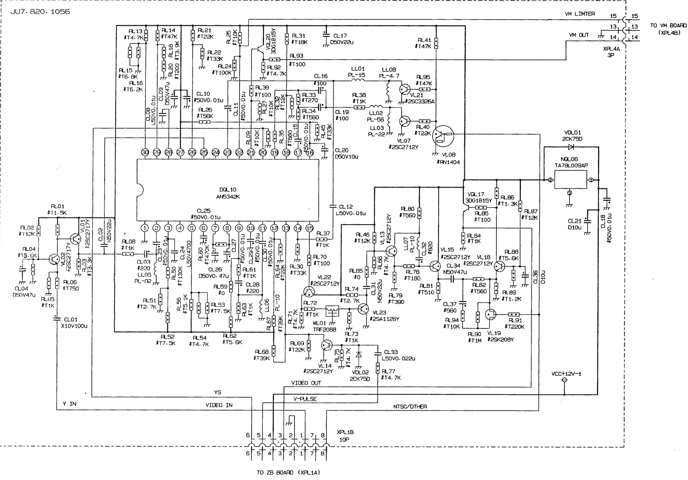
LT BOARD
