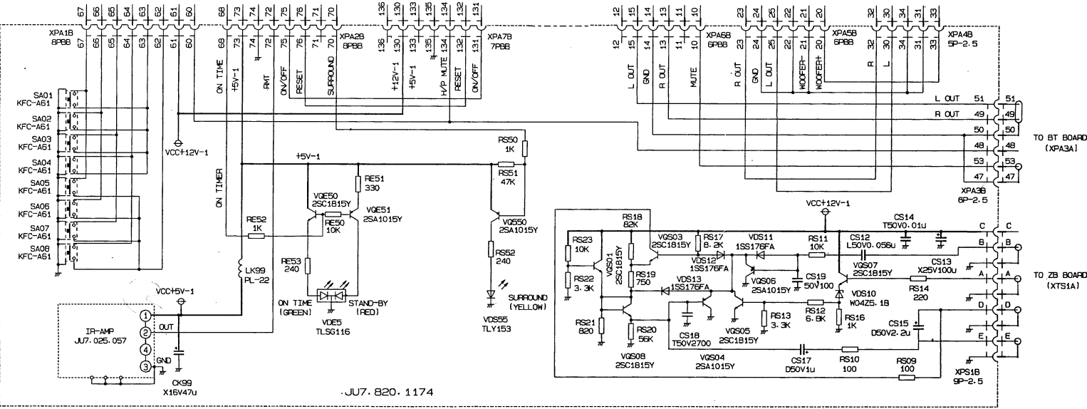
KZ BOARD
