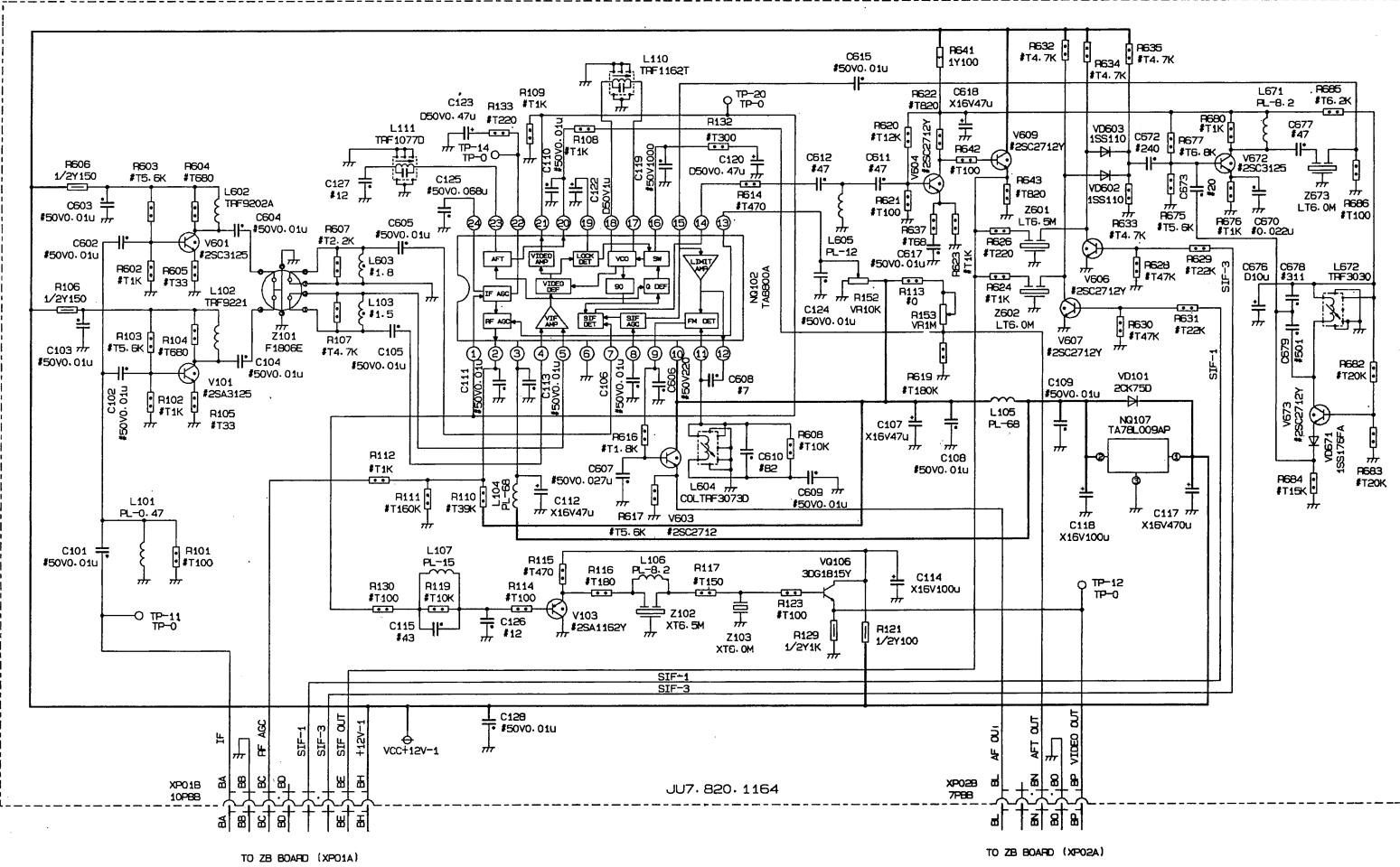
PM BOARD
