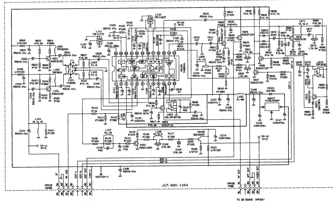
PM BOARD (C3418PN)
