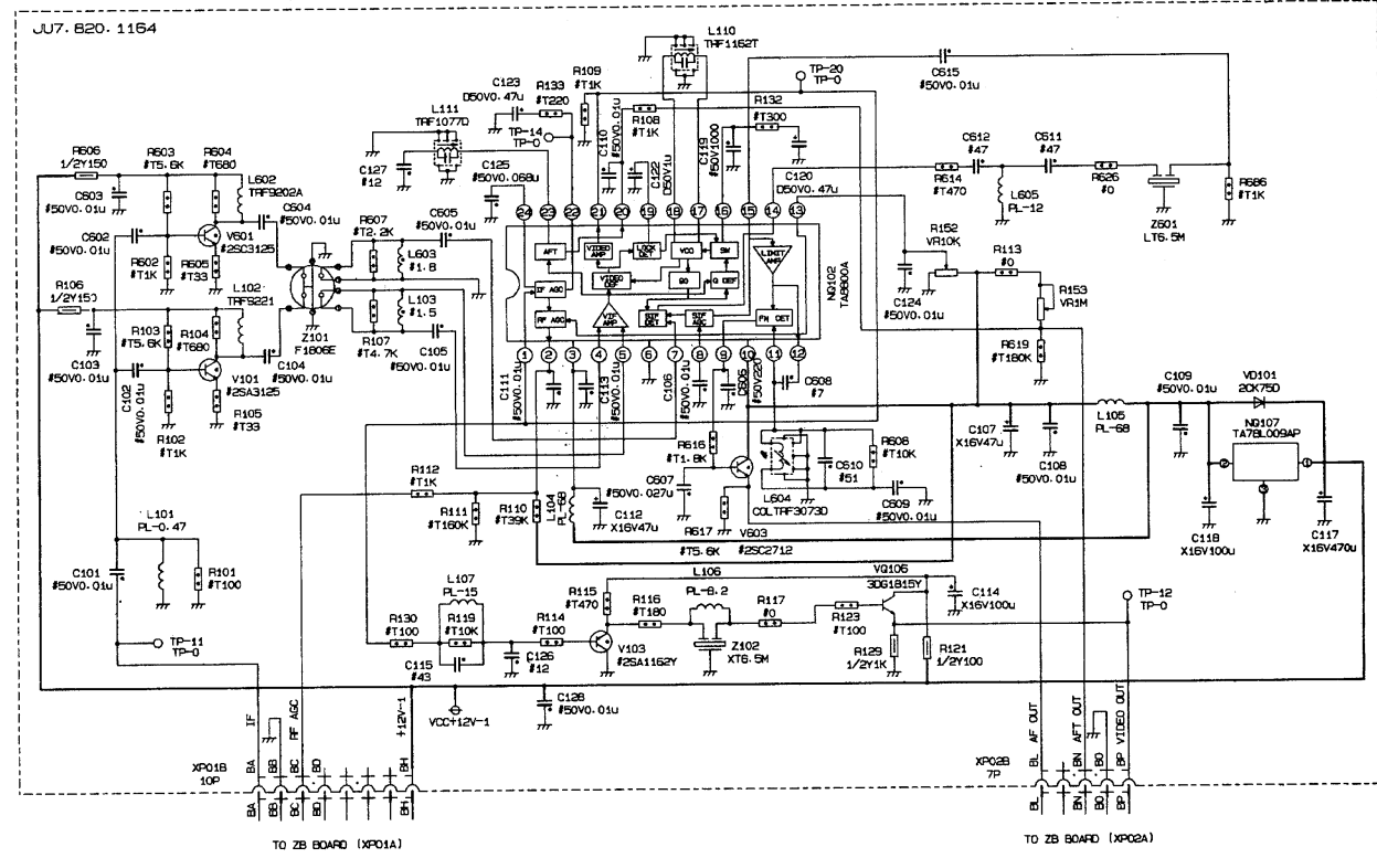
PM BOARD(C3418PS)
