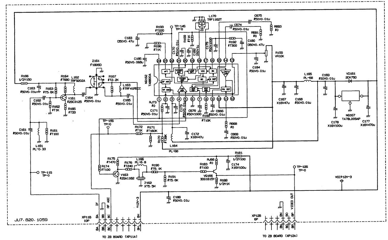
PS BOARD
