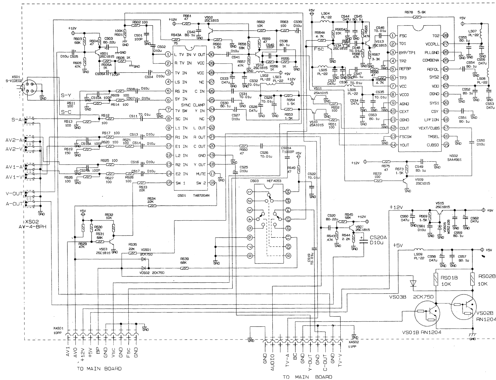
AV-COMB. BOARD
