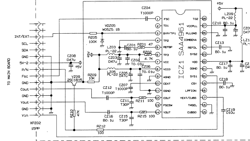
Comb-filter JU7.820.1589
