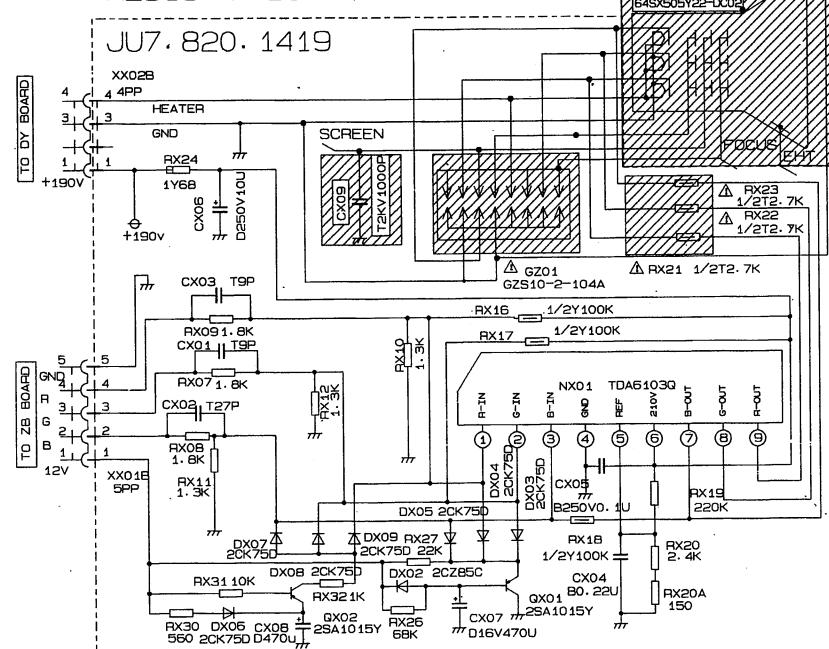
N2516 Y BOARD
