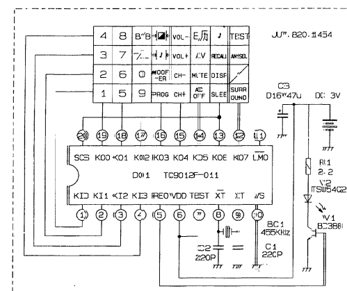
IF REMOTE BOARD
