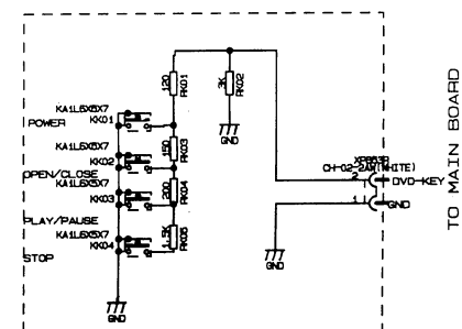
DVD-K BOARD JUC7.820.1035
