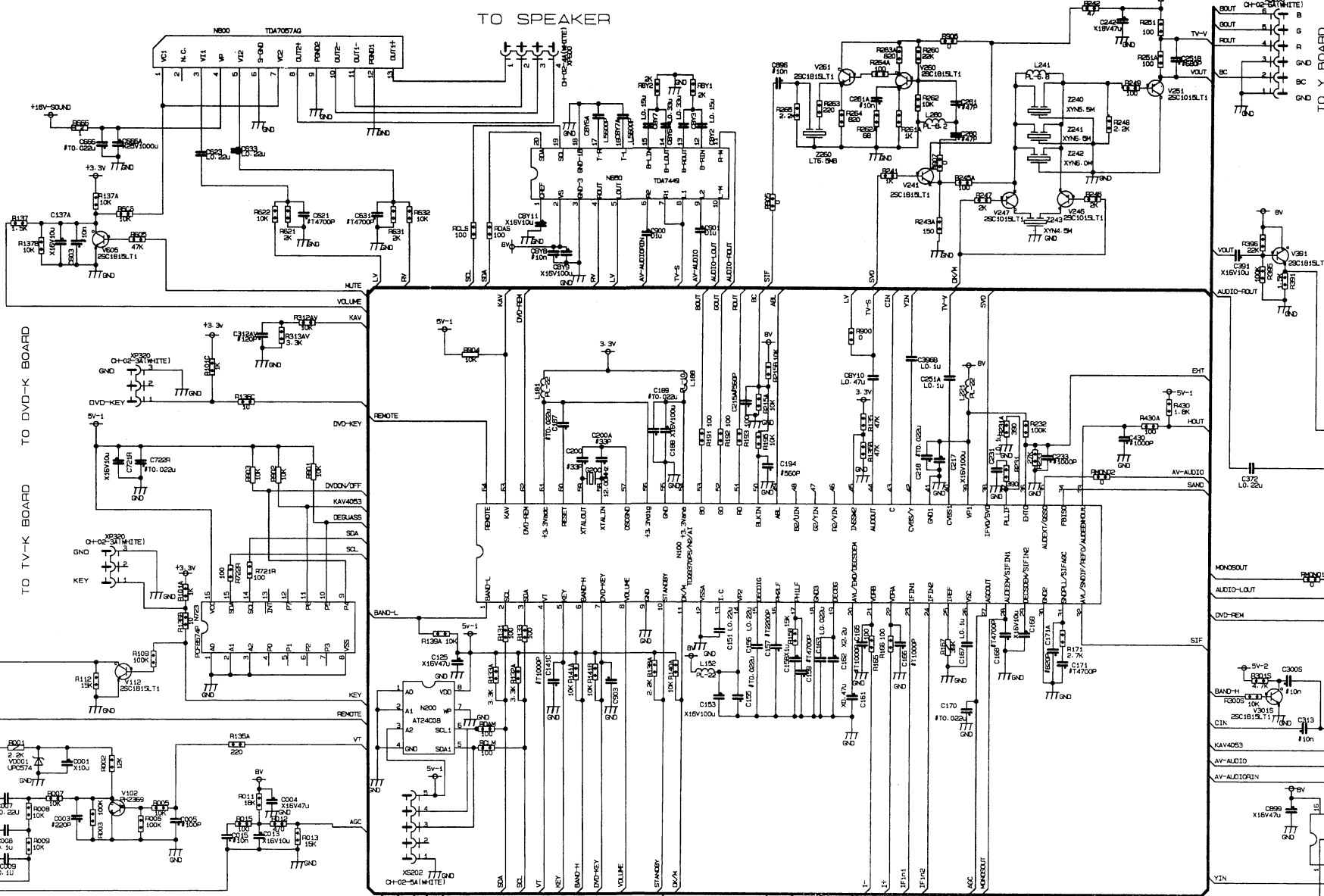
MAIN BOARD JUC7.820.834
