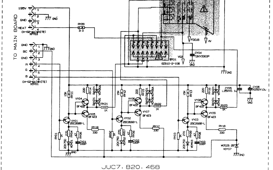
JUC7.820.468
