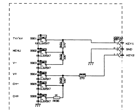
K BOARD
