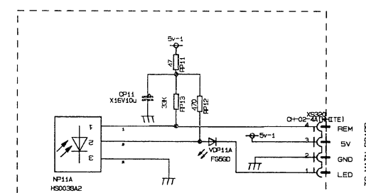
DVD-K BOARD
