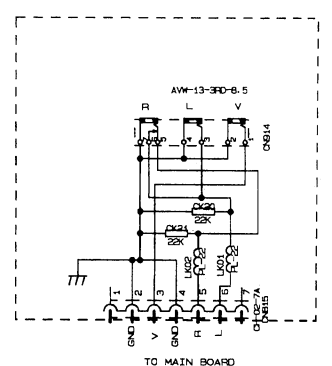
HAY BOARD
