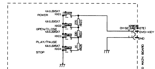
DVD-K BOARD
