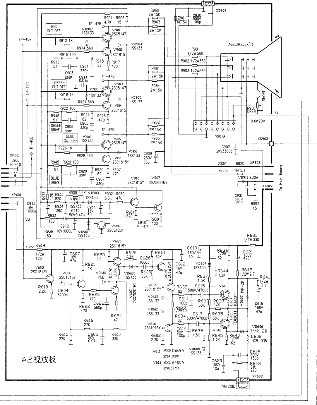
CRT Board
