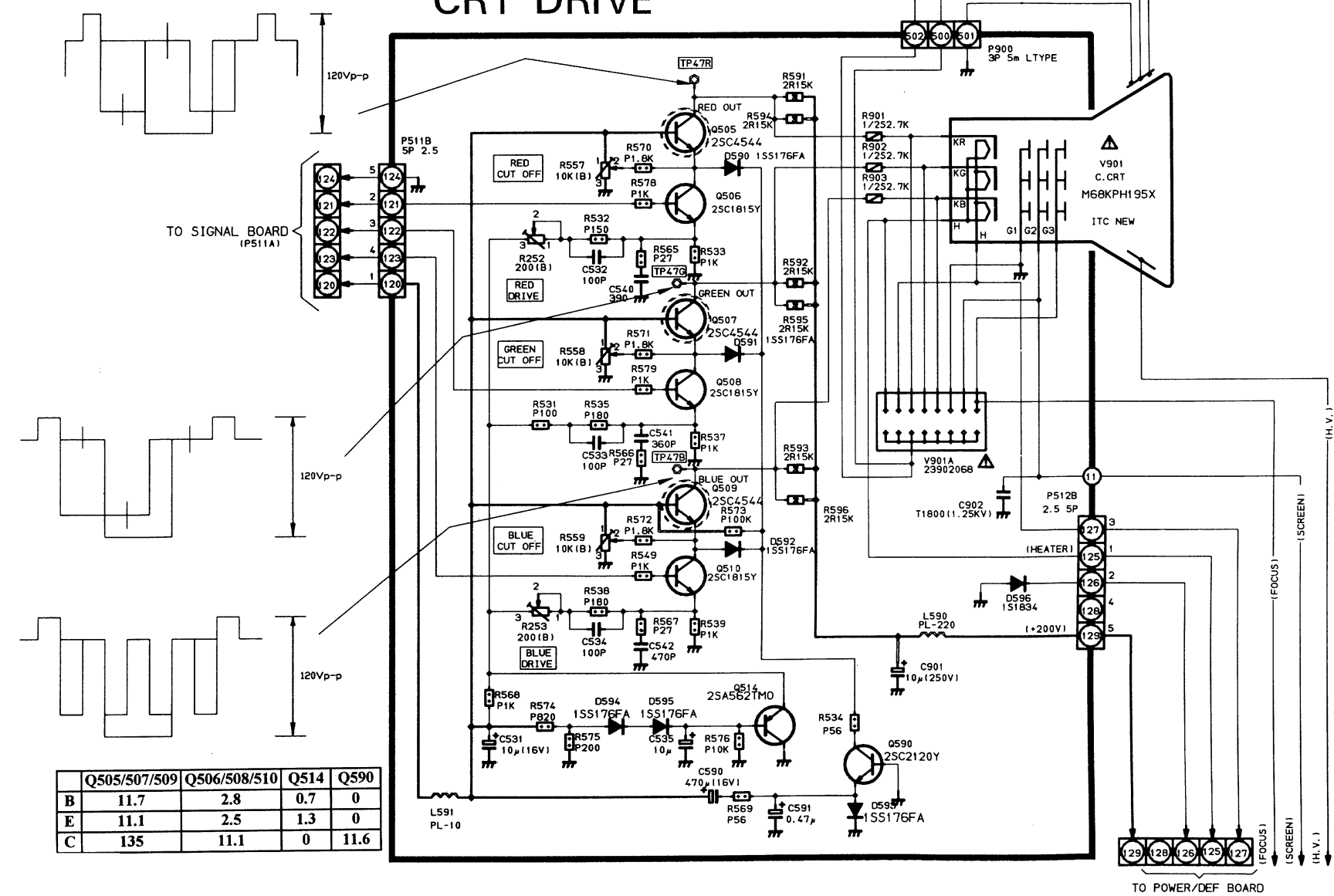
CRT DRIVE
