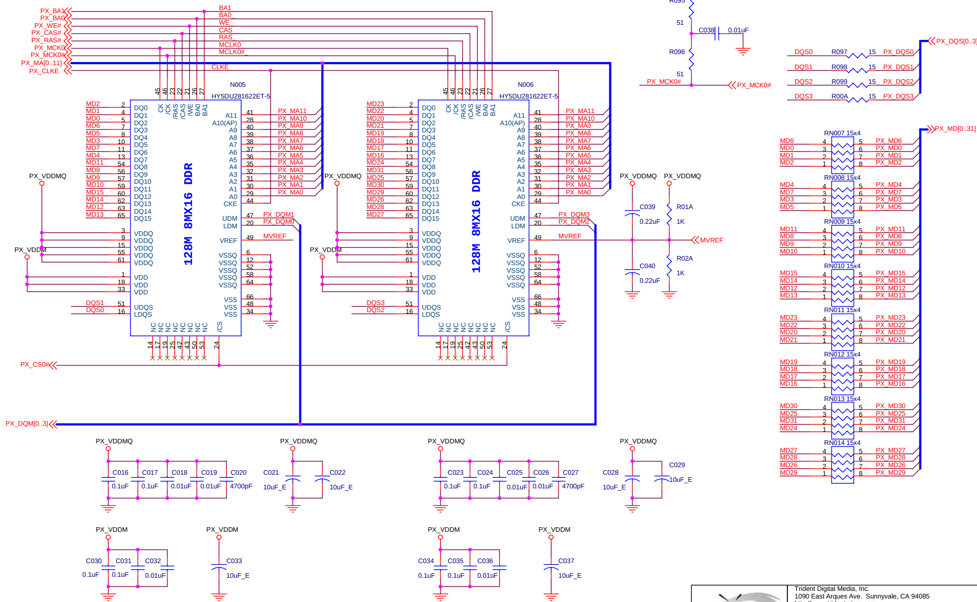
SDRAM DECOUPLING CAPACITORS
