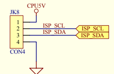
TO MCU
