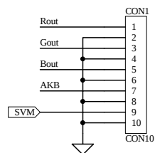
RGB Output for CRT Board
