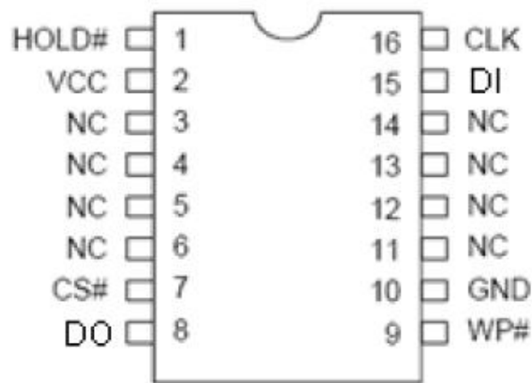
16 - LEAD SOP
