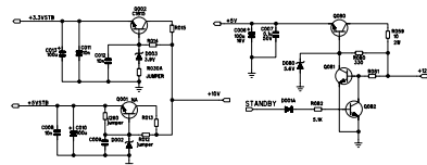
VOLTAGE CONVERSION CIRCUIT
