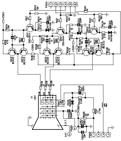
CRT CIRCUIT
