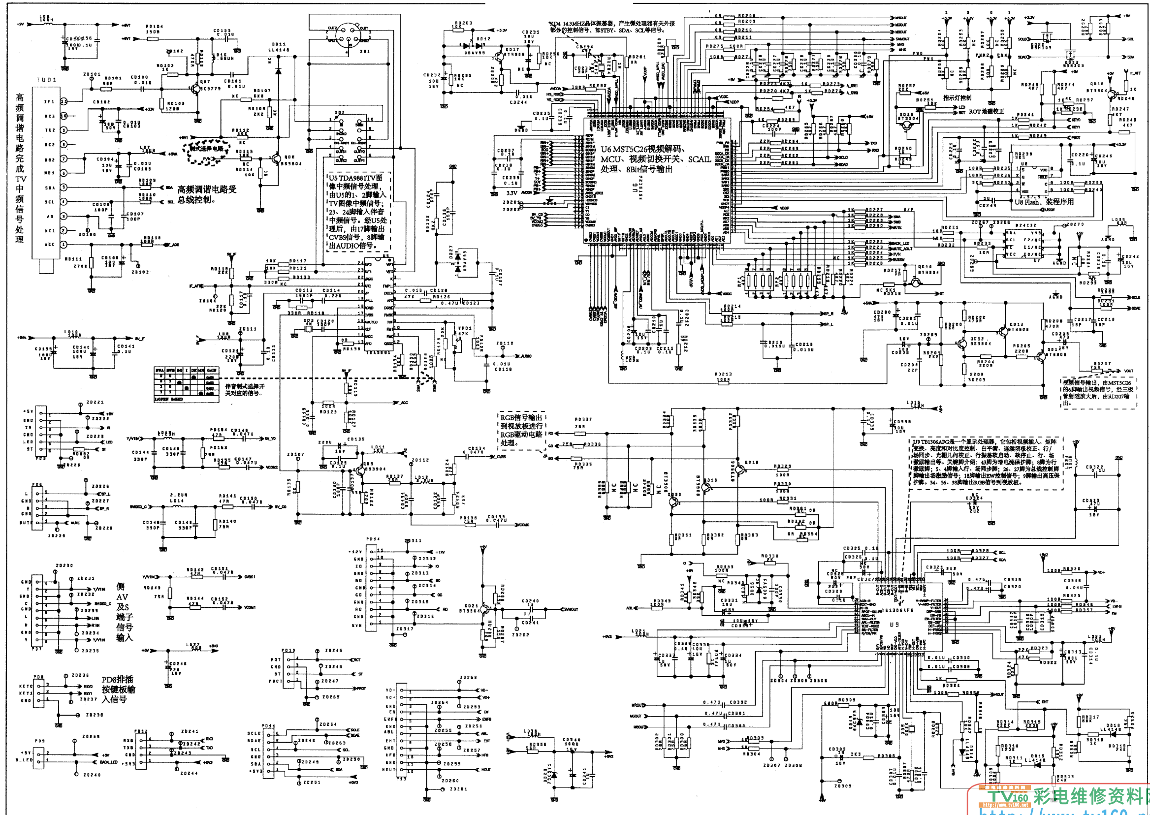
TCL-HD28B03A/HD28H61/HD29276/HD29C06/HD29C81/HD29A71/HD29H61I/HD29C41/HD34C41图2
