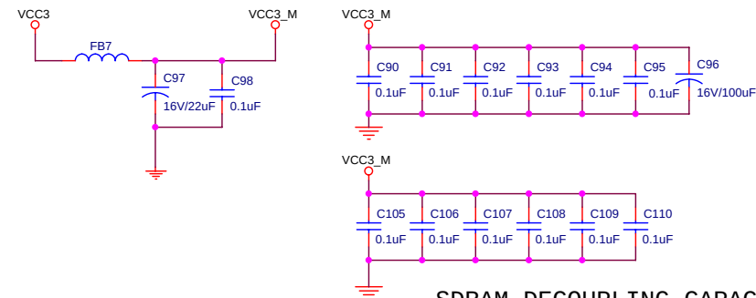
SDRAM DECOUPLING CAPACITORS
