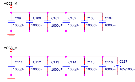
SDRAM DECOUPLING CAPACITORS
