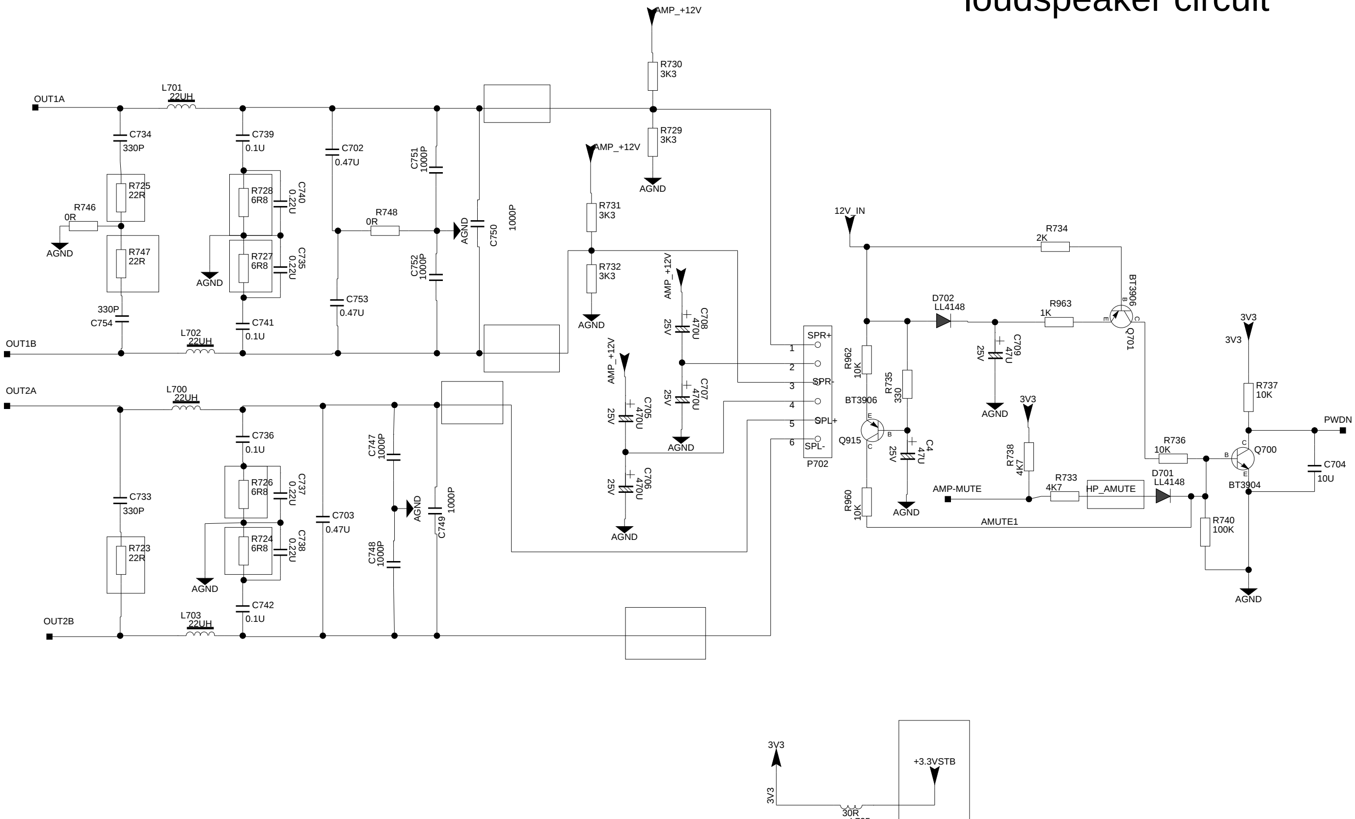
loudspeaker circuit
